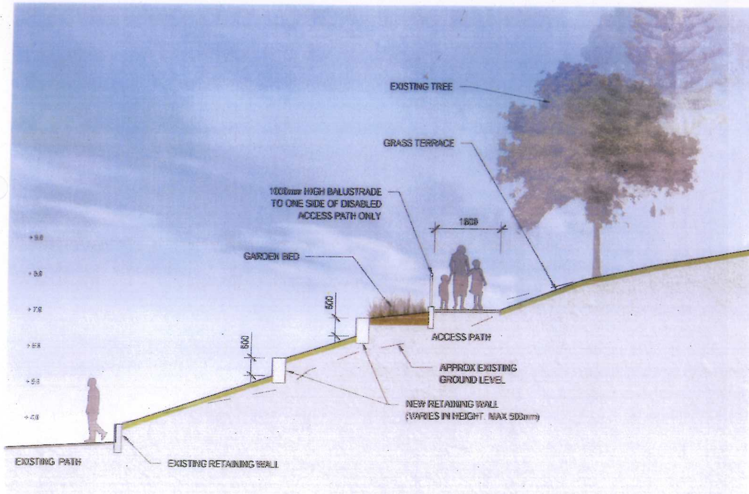
SECTION C
