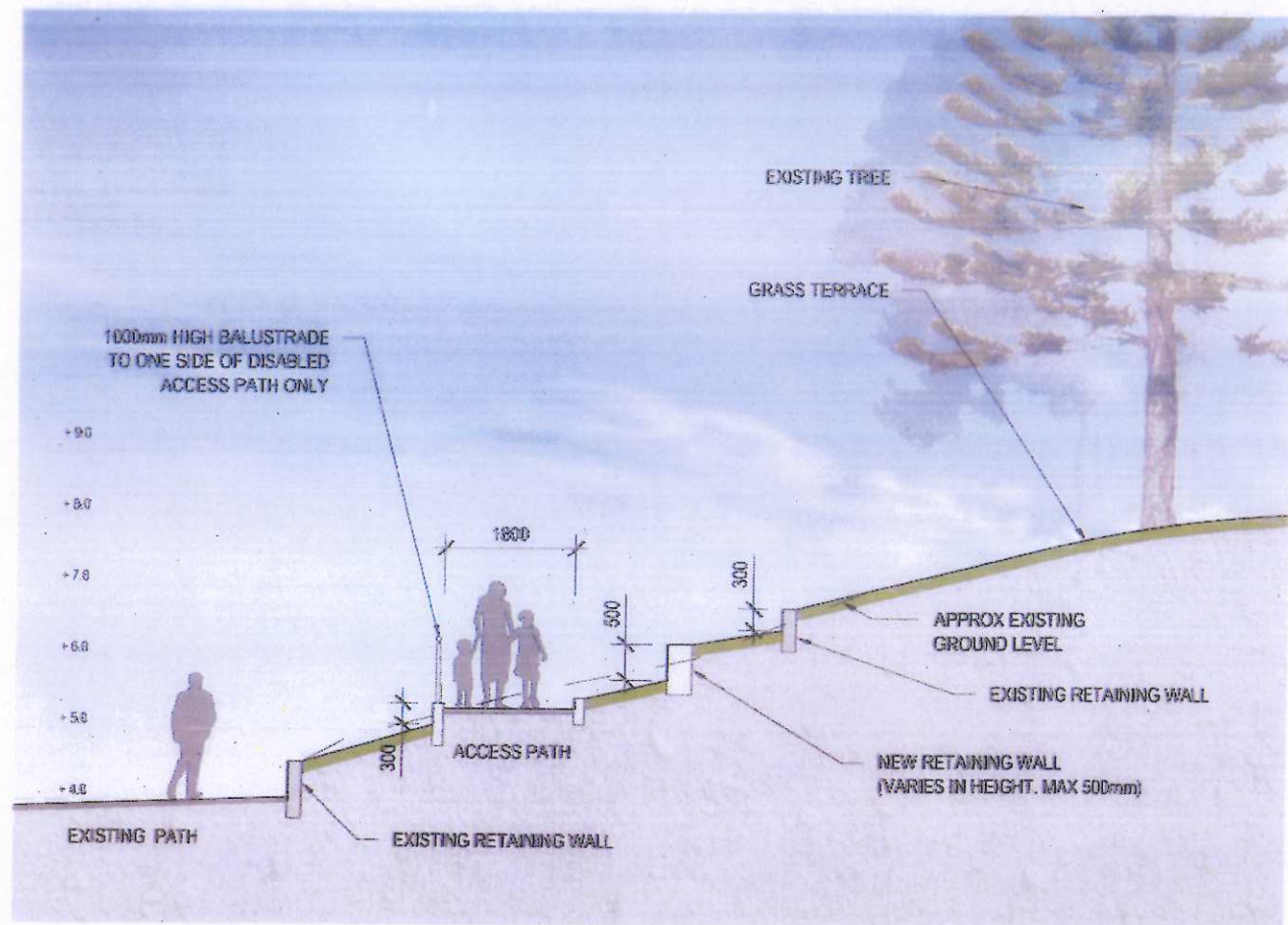
SECTION A
