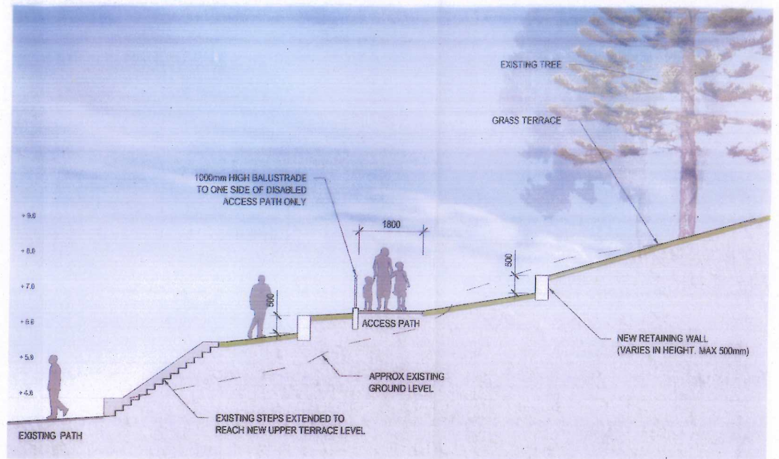
SECTION B
