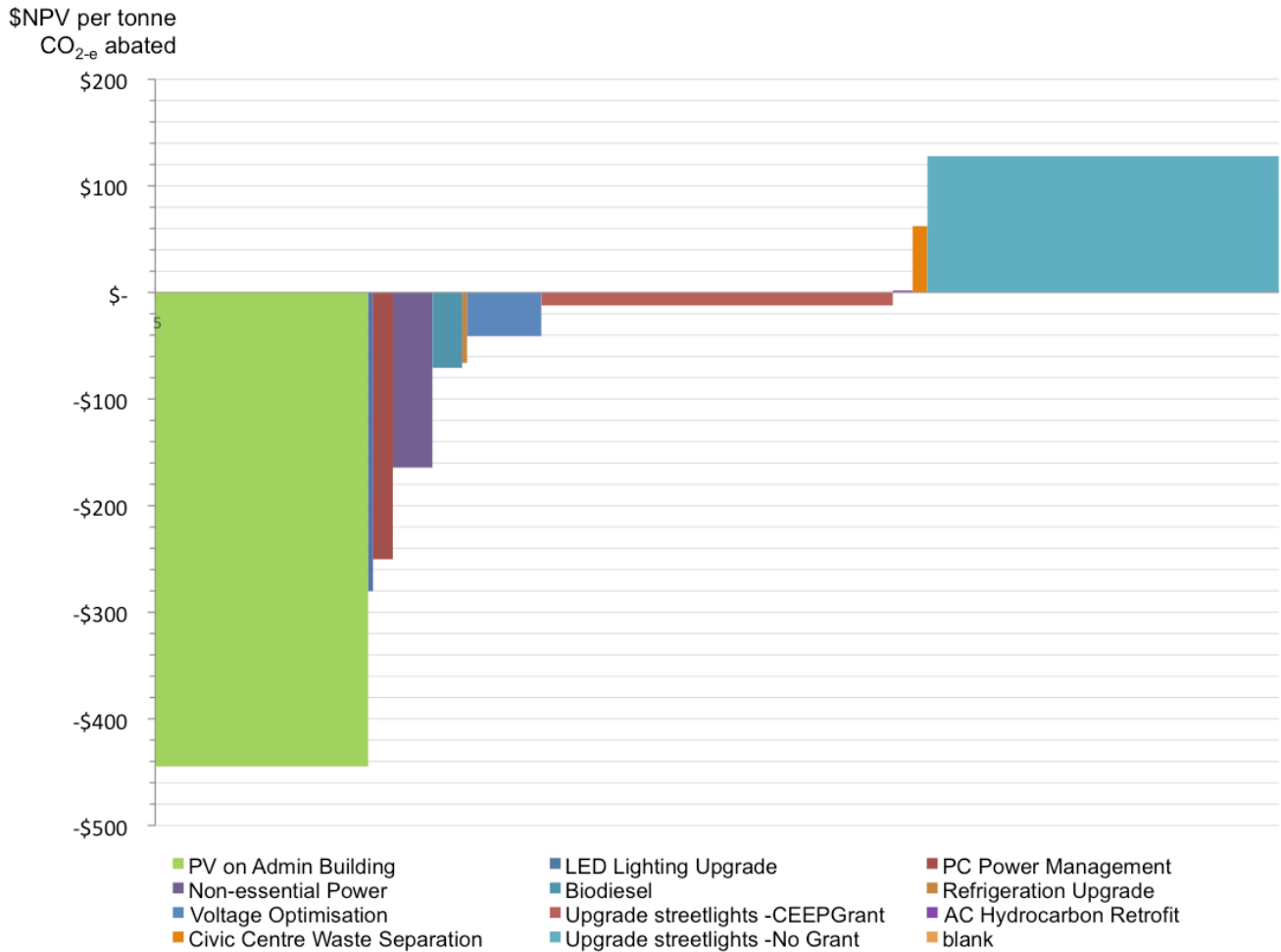
Figure 4: Town of Cottesloe's Marginal Abatement Cost Curve
