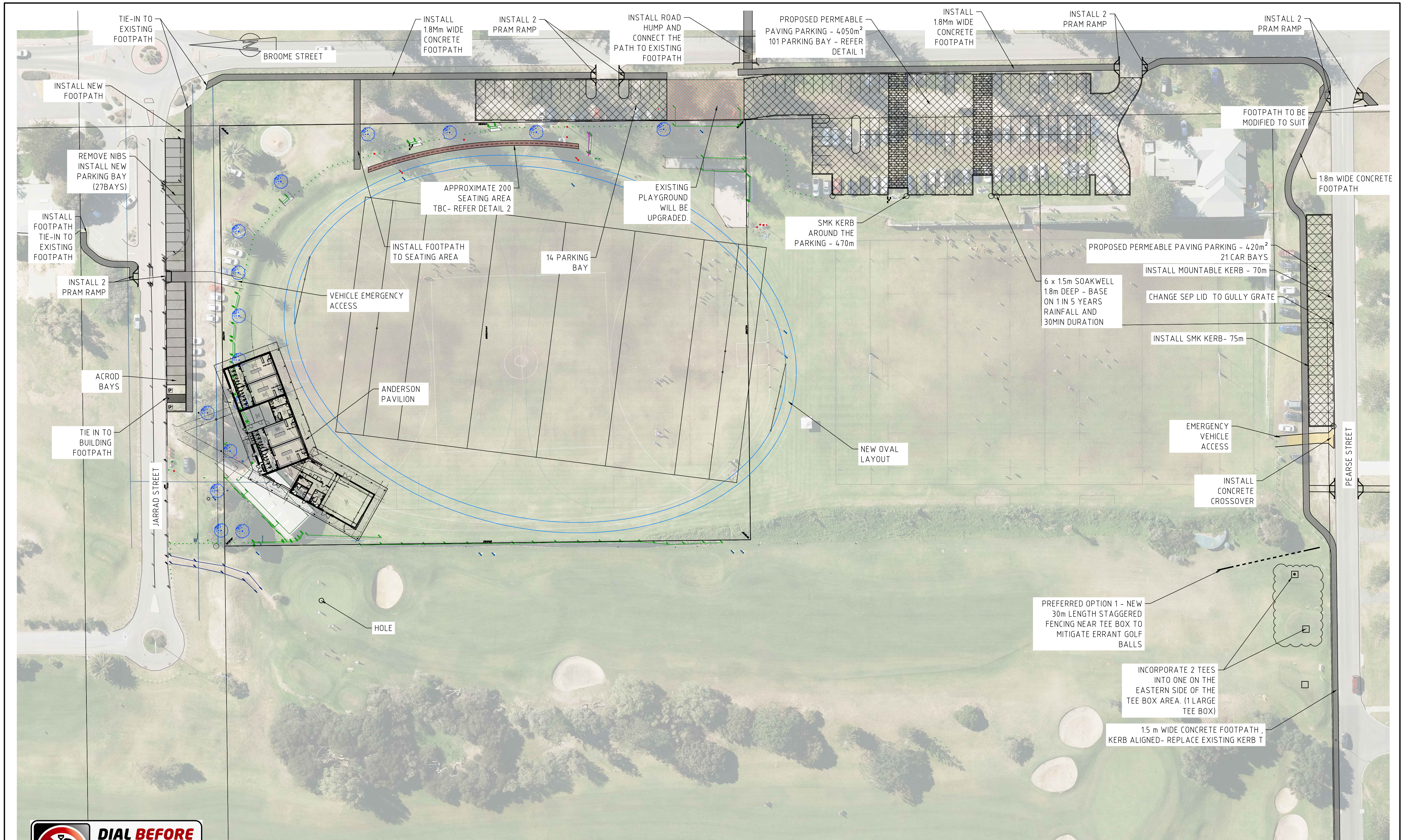
PLAN SCALE 1:500
